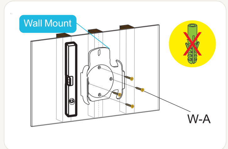
1a.5 Using a Phillips screwdriver, mount the wall mount and fasten it with the provided screws (W-A). Do not use the concrete anchors (W-B) in a wood stud.
