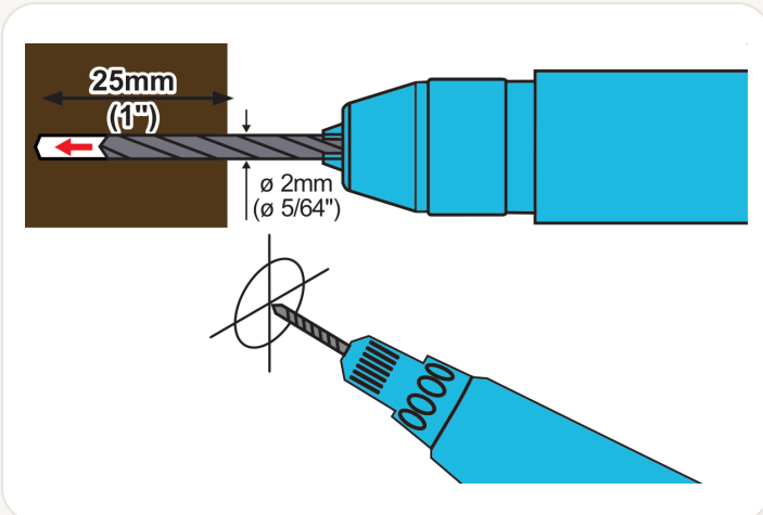
1a.4 Using a power drill and a 5/64 in drill bit, drill pilot holes 5/64 in (2 mm) in diameter and at least 1 in (25 mm) deep.
