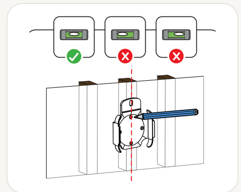
1a.3 Using the wall mount as a template, level it and mark two holes for drilling on the centerline of the stud.
