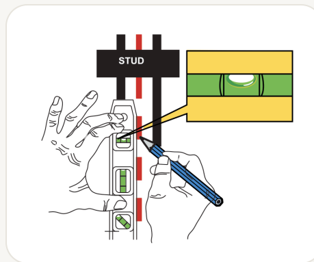
1a.2 Using a level, mark the centerline of the stud.
