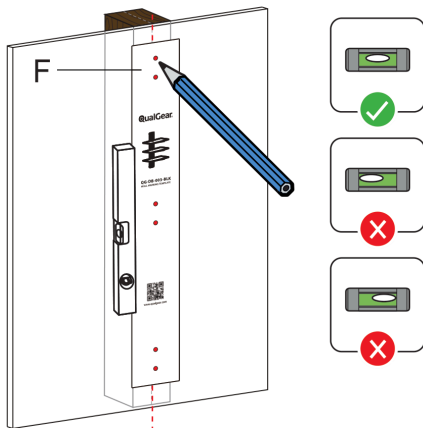
1a.3 Using the marking template (F), mark six holes for drilling on the centerline of the stud.
