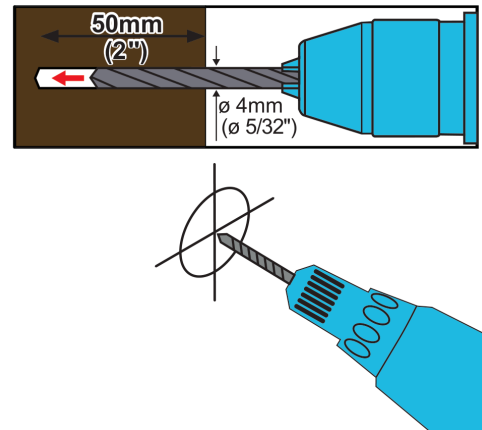
1a.4 Using a power drill and a 5/32 in drill bit, drill pilot holes 5/32 in (4 mm) in diameter and at least 2 in (50 mm) deep.
