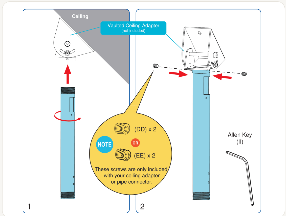
FIG. 1-2 Shown with a vaulted ceiling adapter (not included). The panel numbers match the steps below.
