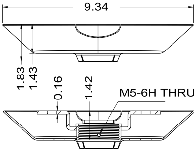
SIDE AND SECTION VIEWS
